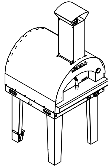
Isometric View
